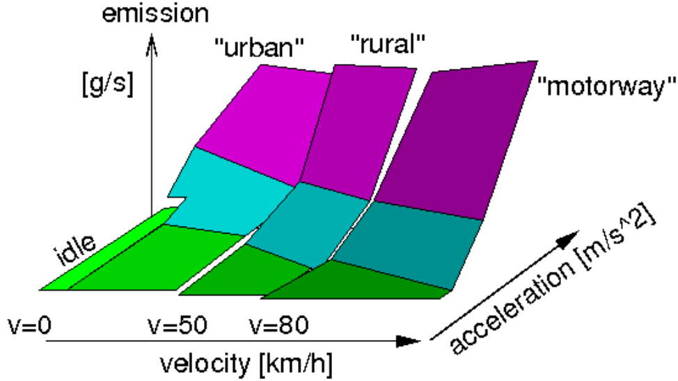
Figure 3: Sketch of the generic piece-wise linear model dependence of the emissions on the velocity-acceleration regions.
